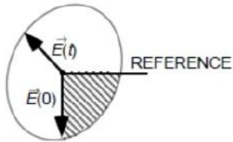
Figure 2 — Elliptically polarized field
